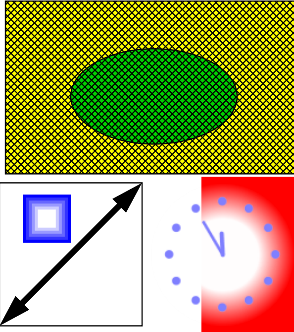
Figure 1: Test image
